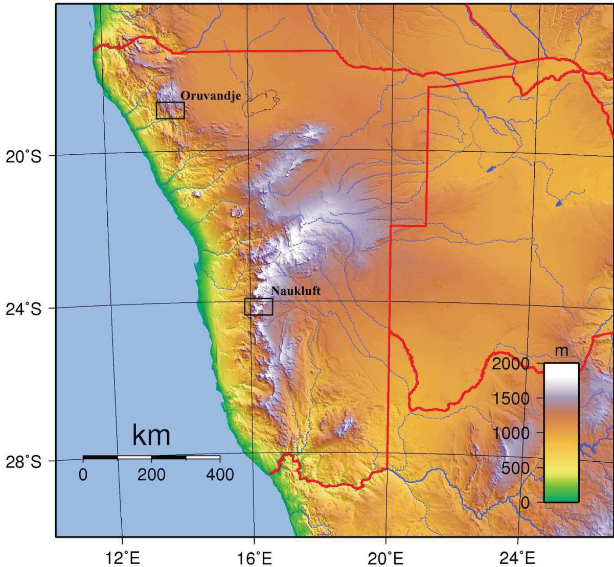
Figure 1. Relief map of Namibia showing the area of Kaokoland Tufa deposits (black rectangle at Oruvandje on the southern flanks of the Joubert Mountains) west of Etosha Pan (dotted ovoid outline) and in the Naukluft Mountains. Note the positions of the tufa deposits at high altitudes along the edge of the «Great Escarpment» which separates the deeply incised coastal strip, from the flatter interior of the continent.
