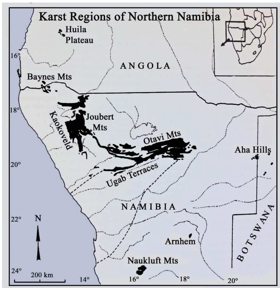
Figure 2. Distribution of the Otavi Dolomites and other Proterozoic carbonates (black areas) in Namibia and Angola. The southern flanks of the Joubert Mountains and the Naukluft Mountains were the sites of extensive tufa deposition during the Late Neogene and Quaternary.
