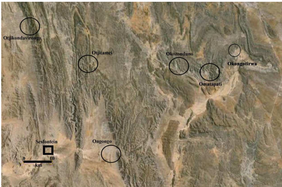
Figure 4. The main areas in Kaokoland, north and east of Sesfontein, at which cascade tufas have been mapped (Map modified from Google Earth).
