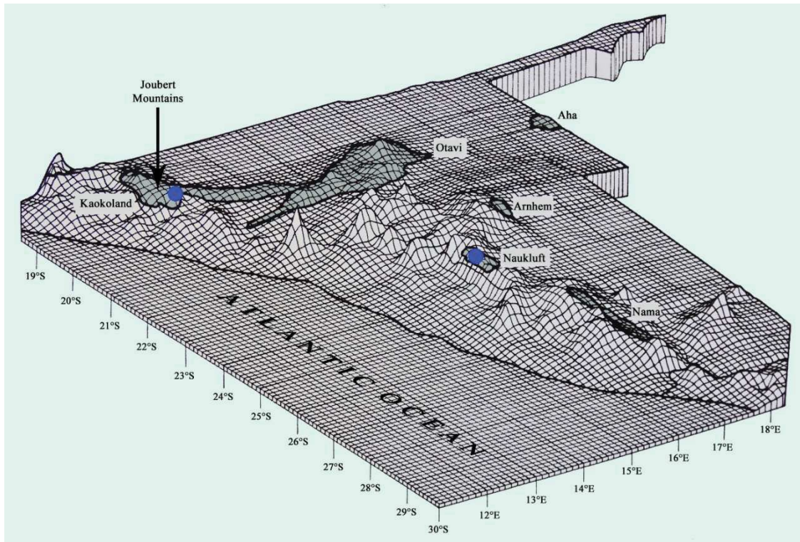
Figure 3. Oblique relief map of Namibia showing the distribution of dolomites (light blue) and extensive tufa deposits (dark blue). The tufa deposits formed preferentially at high altitudes along the edges of the Great Escarpment indicating the essential roles that climate and bedrock substrate played in their genesis.
