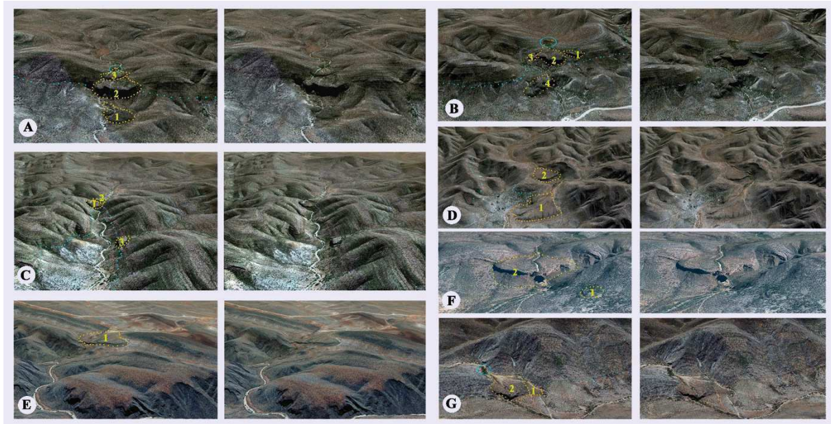
Figure 5. Stereo oblique views of cascade tufa lobes in Kaokoland showing the characteristic geomorphology that they produce. A) Okapiku (3 lobes), B) Okongwe (4 lobes), C) Orutjene (2 lobes) and Okovanatje (1 lobe), D) Omatapati (2 lobes of very different ages), E) Otjimatei (1 huge lobe), F) Okongotirwa (2 lobes), and G) Otjikondavirongo (2 lobes of different ages). The blue dots follow the contact between carbonate rocks above and relatively impervious sericitic rock below. The blue ovals encircle resurgences upstream from the tufa lobes. The dimensions, co-ordinates and altitudes of the lobes are provided in Table 1 (images modified from Google Earth).
